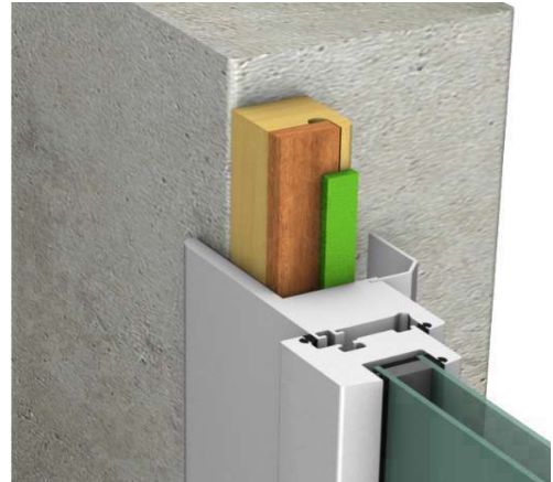
Illustration 56: Tremco-Ilbruck 3D objects for joinery
