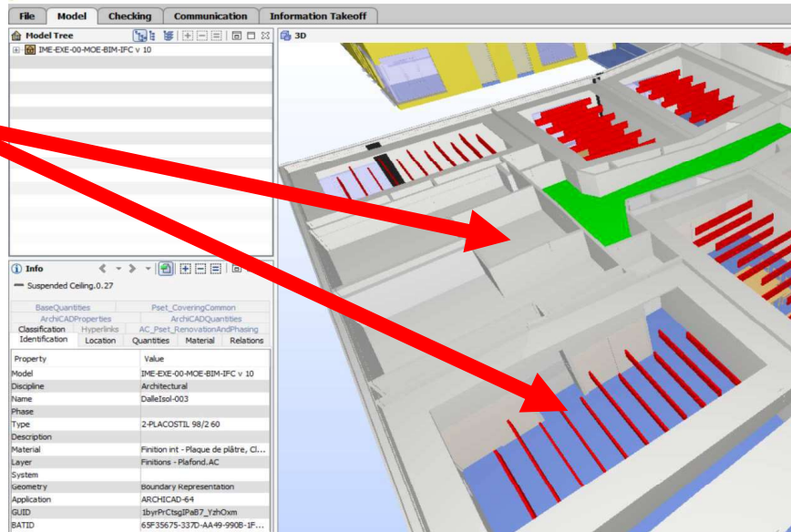
Illustration 37: visualisation of different types of false ceilings
