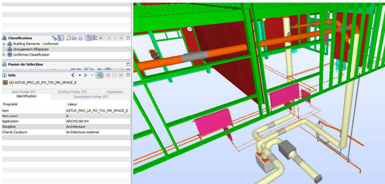
Illustration 52: identification of blockout
